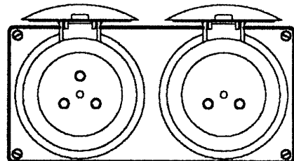
C3DF-44 Tomas: 2 x 40 Amp.
