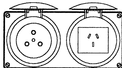
C3DF-41 Tomas: 1 x 40 + 1 x 10 Amp.
