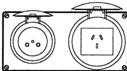
C3DF-21 Tomas: 1 x 20 + 1 x 10 Amp.
